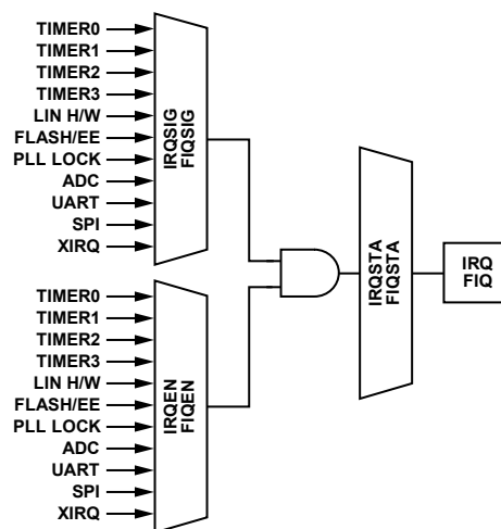
Figure 29. Interrupt Structure
