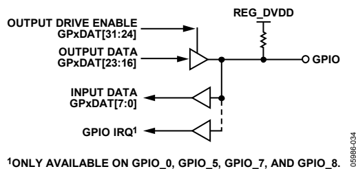
Figure 34. ADuC7032-8L GPIO
